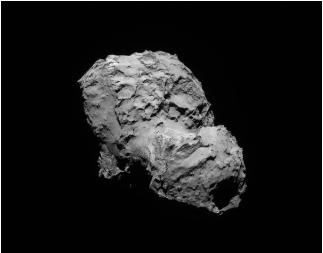
Comet 67P/Churyumov-Gerasimenko photographed on 5AUG14.
